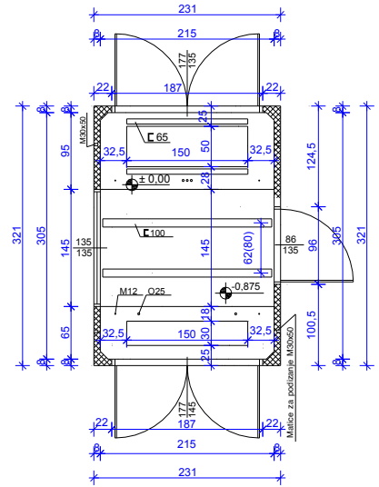
EBB KTS1 1x630(1x1000) kVA, 10/0,4kV
